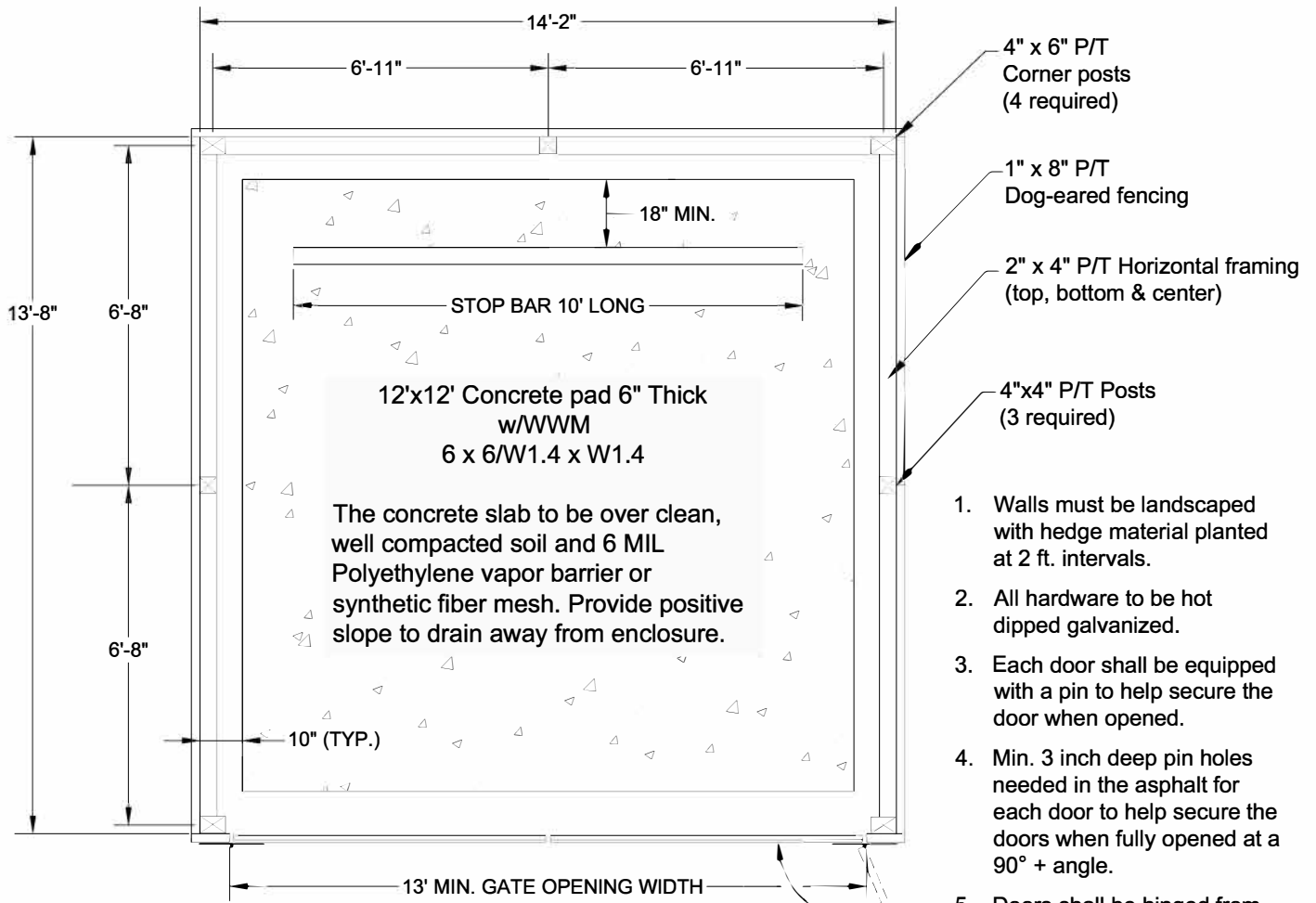
PLAN VIEW
