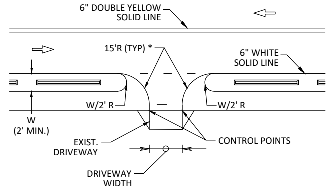
DETAIL 3 USE AT EXISTING DRIVEWAY OPENINGS N.T.S.
