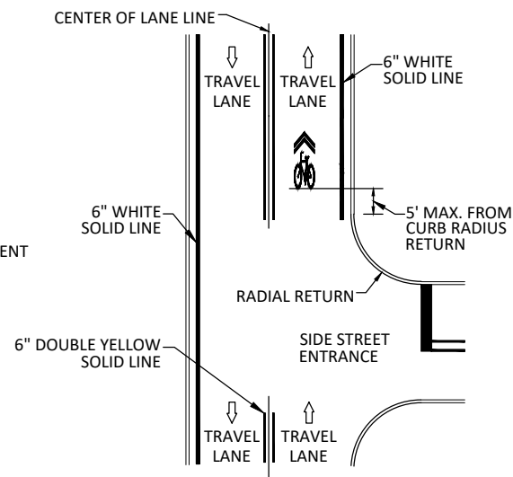
DETAIL 2 SHARED LANE MARKING PLACEMENT AT FAR SIDE OF THE INTERSECTION N.T.S.
