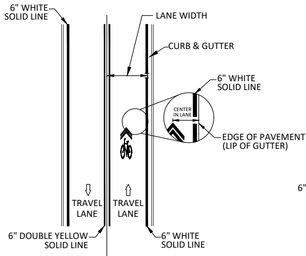
DETAIL 1 SHARED LANE MARKING USE AT LANE WIDTH ≤ 14' N.T.S.
