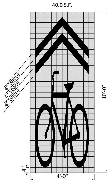
DETAIL 2 SHARED LANE MARKING WITH GREEN BACKGROUND N.T.S.
