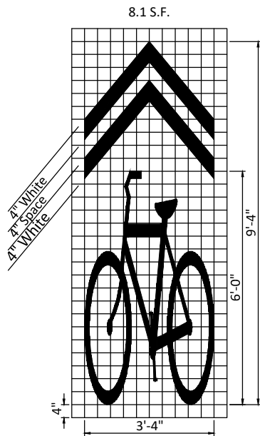
DETAIL 1 SHARED LANE MARKING N.T.S.
