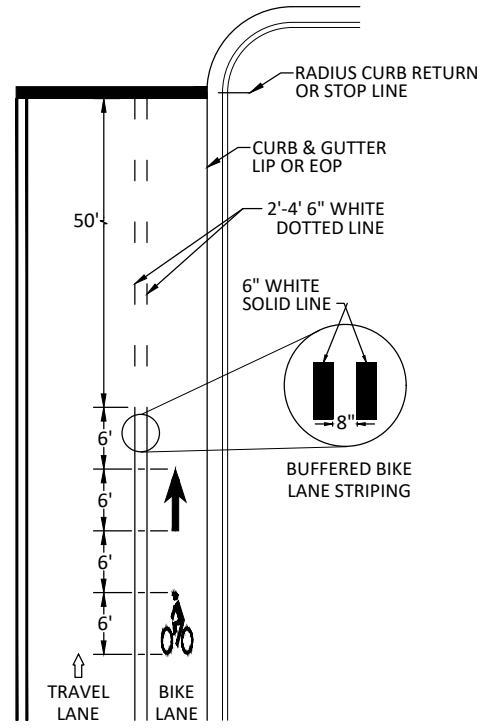
DETAIL 3 BIKE LANE MARKING PLACEMENT AT INTERSECTION N.T.S.
