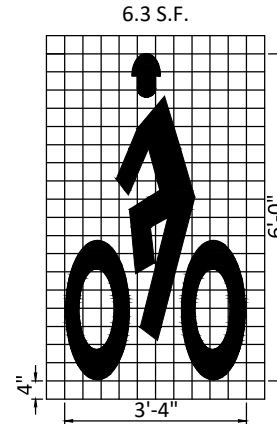
DETAIL 3 HELMETED BICYCLIST SYMBOL N.T.S.
